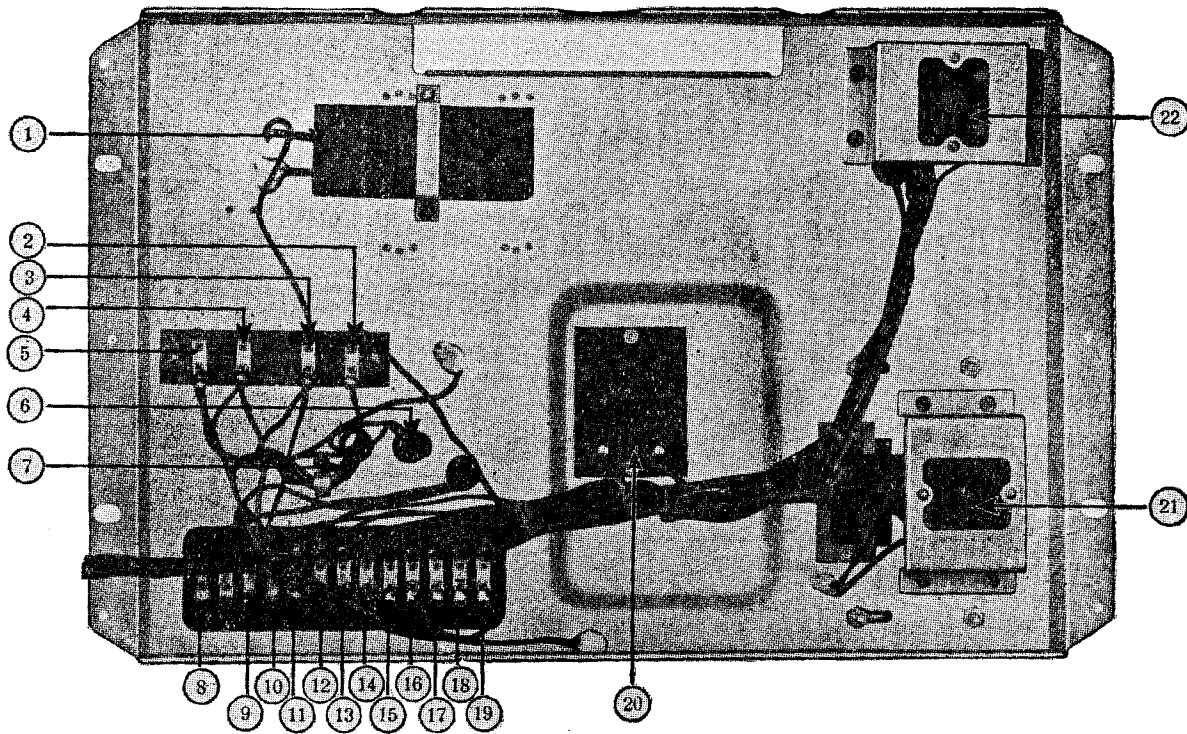
Interior View of Model 220 Power Unit
